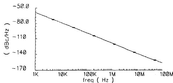
Fig. 7. Phase noise.
