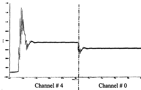
Fig. 8. VCO control voltage during channel switching.
