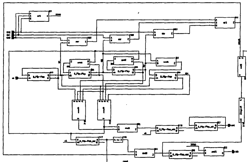
Fig. 4. Program and pulse swallow counter.
