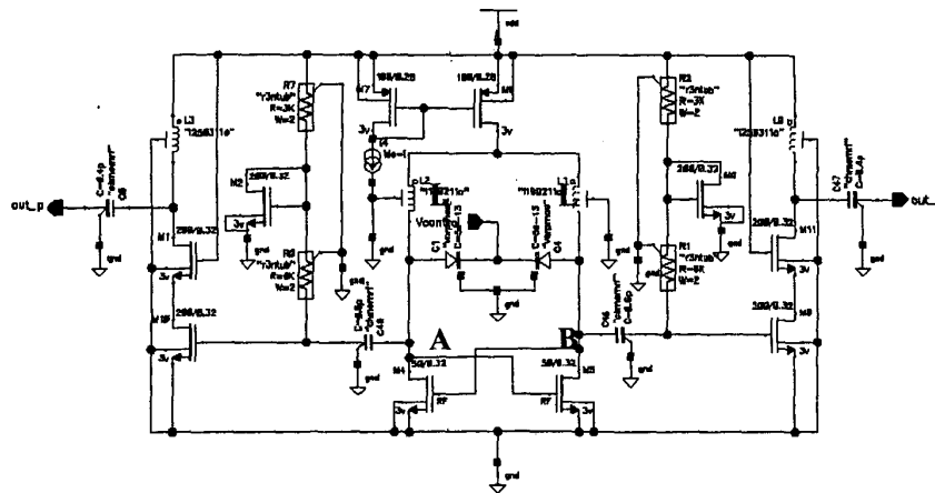
Fig.2. VCO with buffer amplifier.
