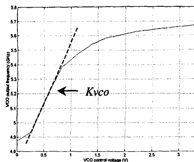
Fig. 6. VCO tuning range.
