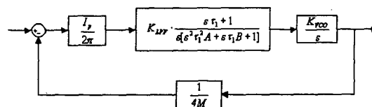
Fig. 5. Linearized PLL Model.
